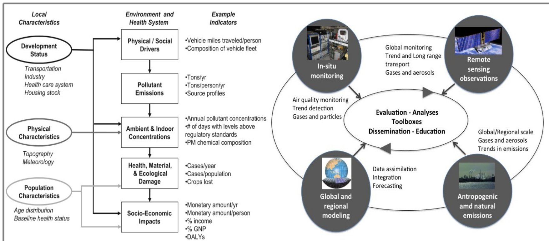
Figure 1. Left: Chain of environmental indicators used to gauge health consequences of environmental hazards: from drivers to impacts (Bell et al., 2011). Right: Key elements of an air quality monitoring, analysis and forecast system .
